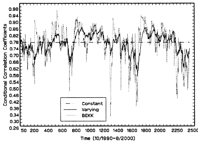
Figure 6. Conditional-Correlation Coefficients of (F, P).
