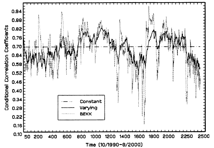
Figure 7. Conditional-Correlation Coefficients of (F, U).
