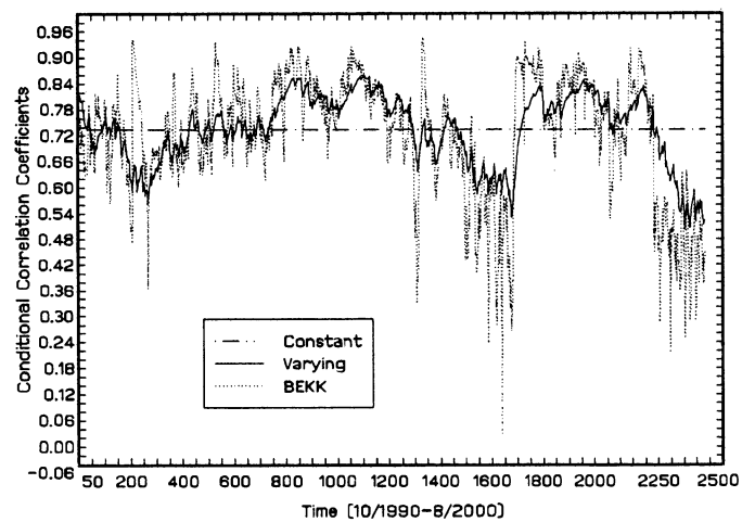
Figure 8. Conditional-Correlation Coefficients of (P, U).
