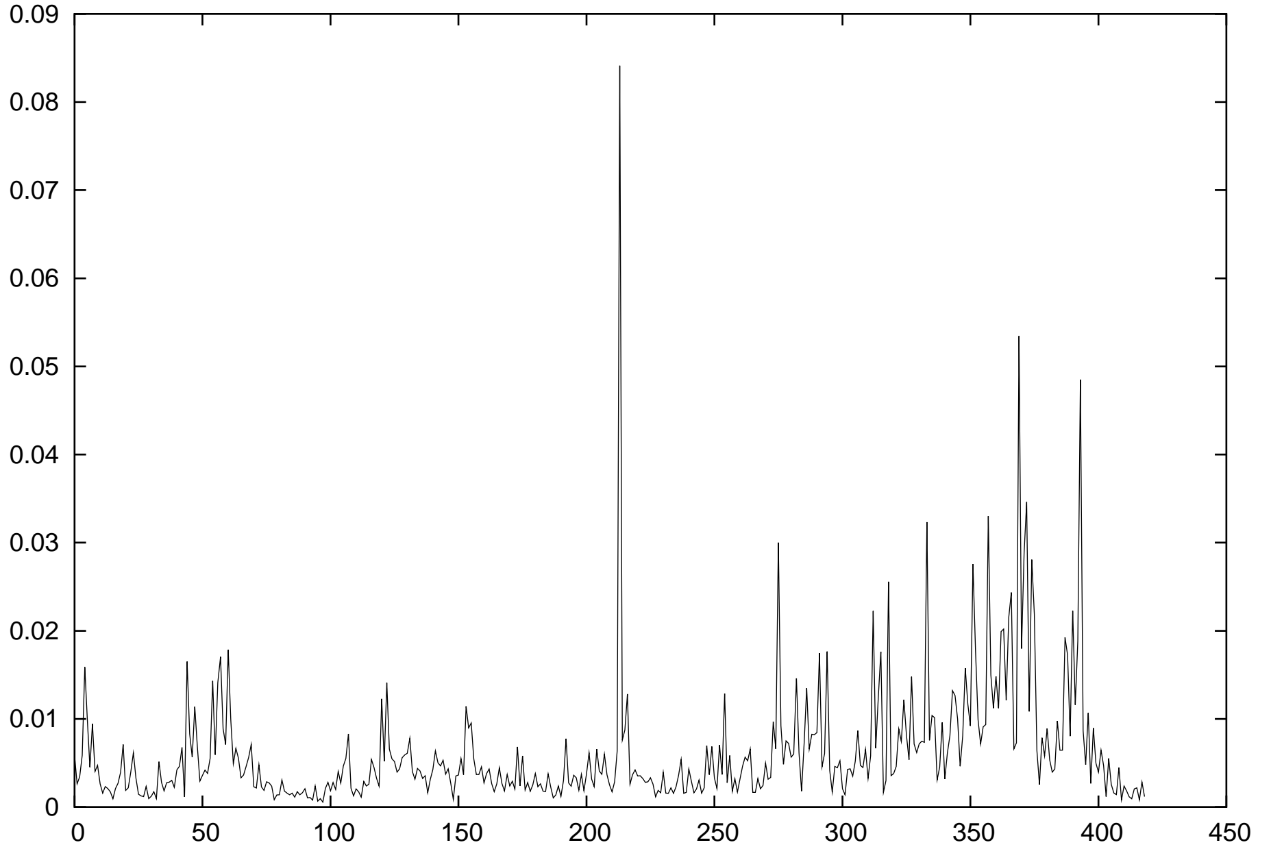
Monthly RV
