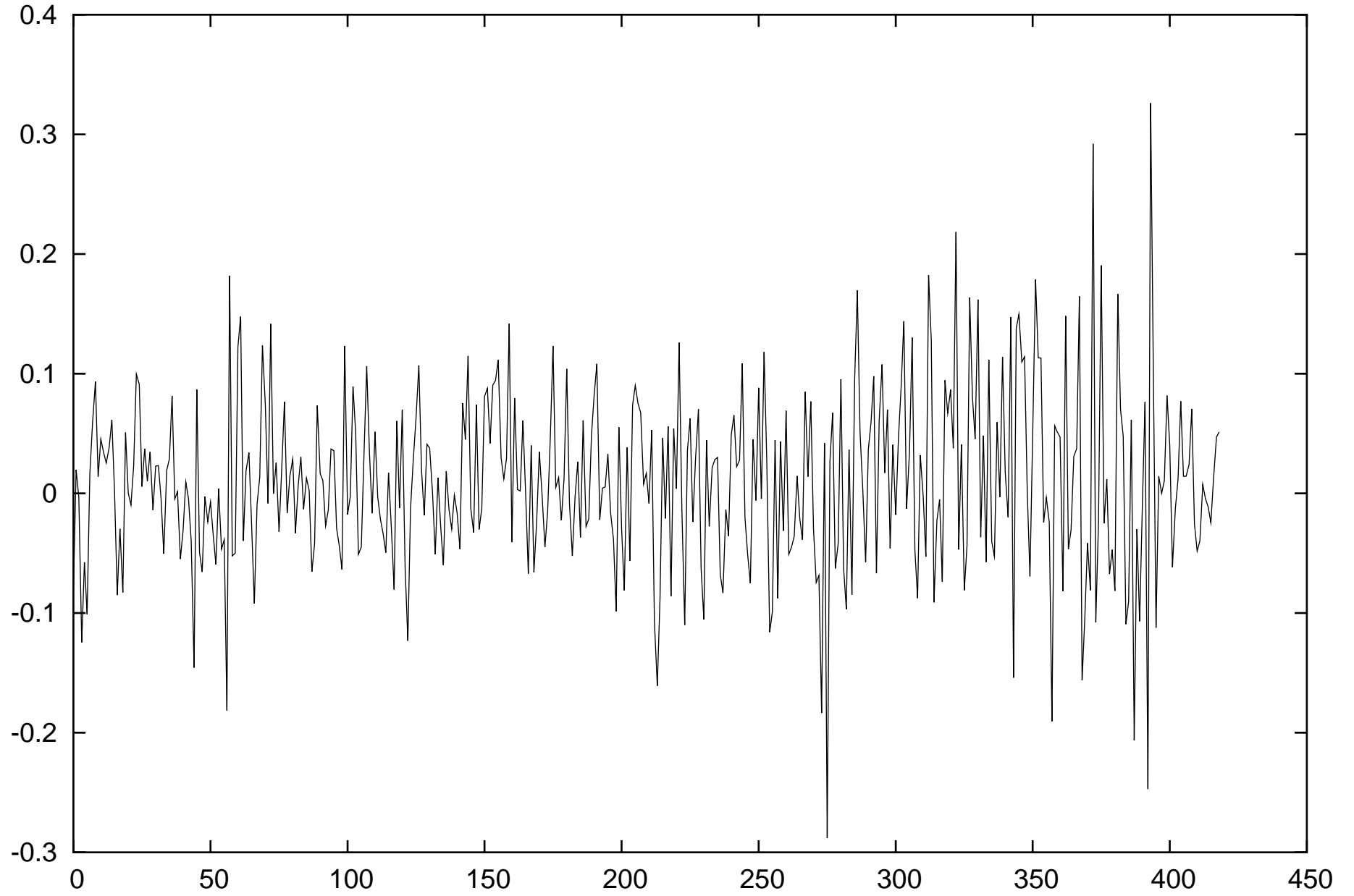
Monthly returns
