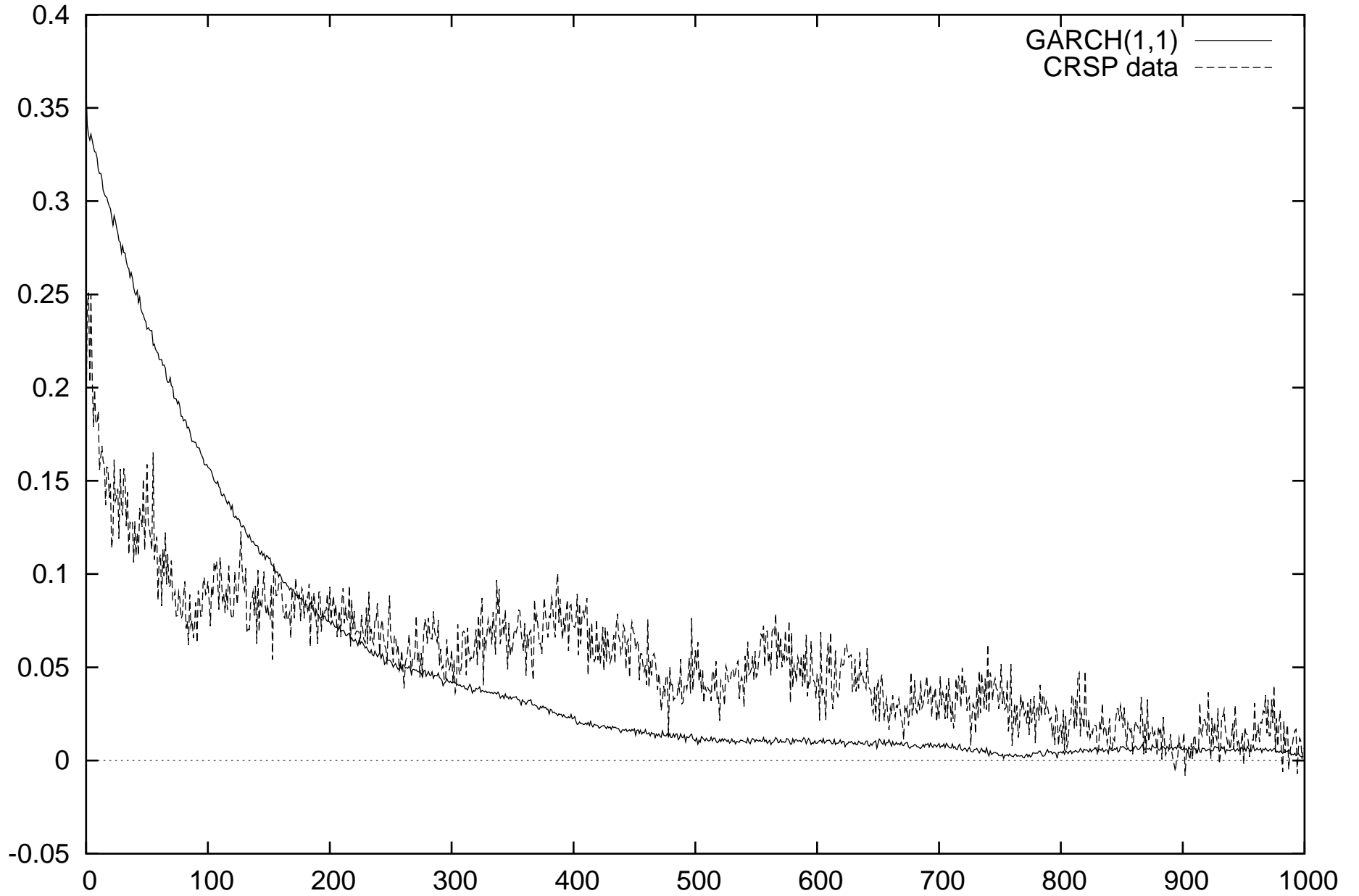
ACF of absolute value of returns, model and data
